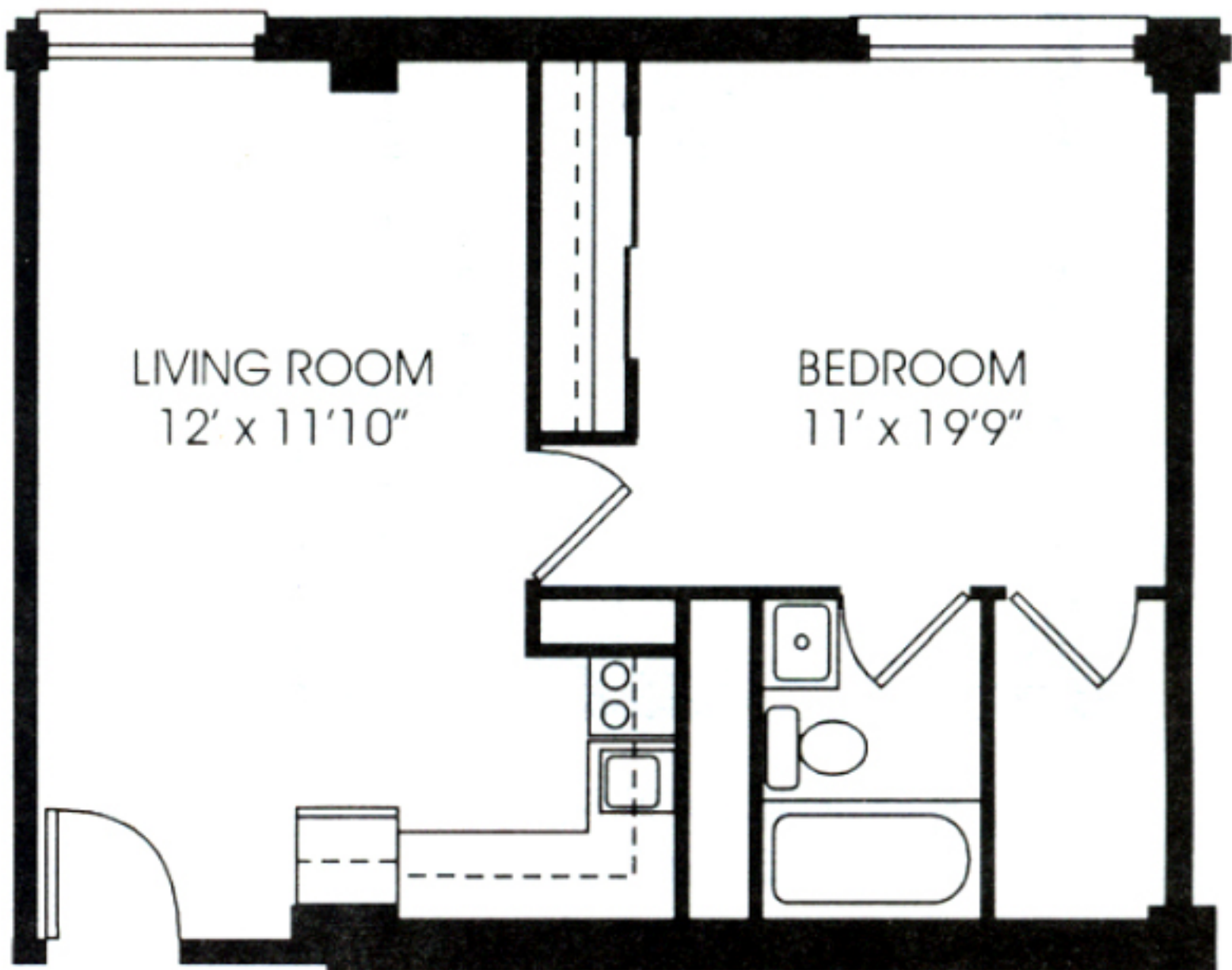
1 BEDROOM 550 SQ. FT. 14 UNITS
